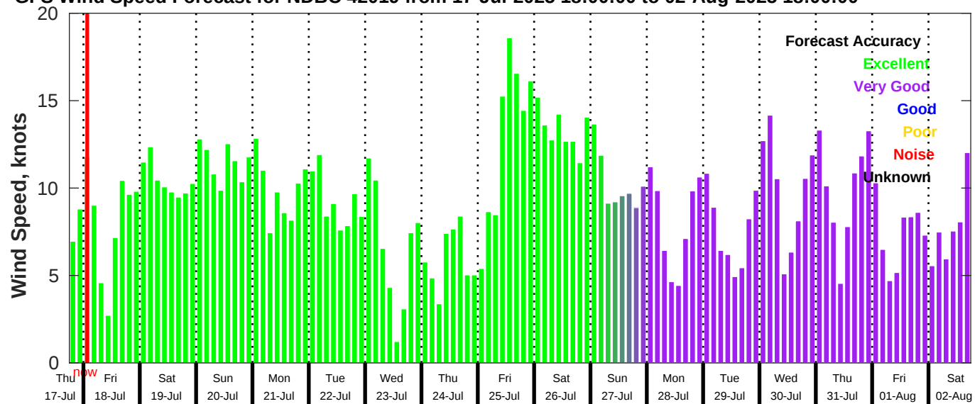
GFS Wind Speed Forecast for NDBC 42019 from 17-Jul-2025 18:00:00 to 02-Aug-2025 18:00:00
