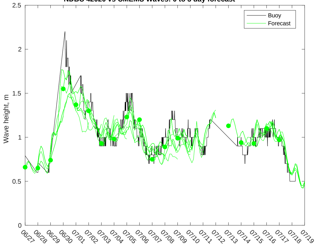
NDBC 42020 vs CMEMS Waves: 0 to 3 day forecast
