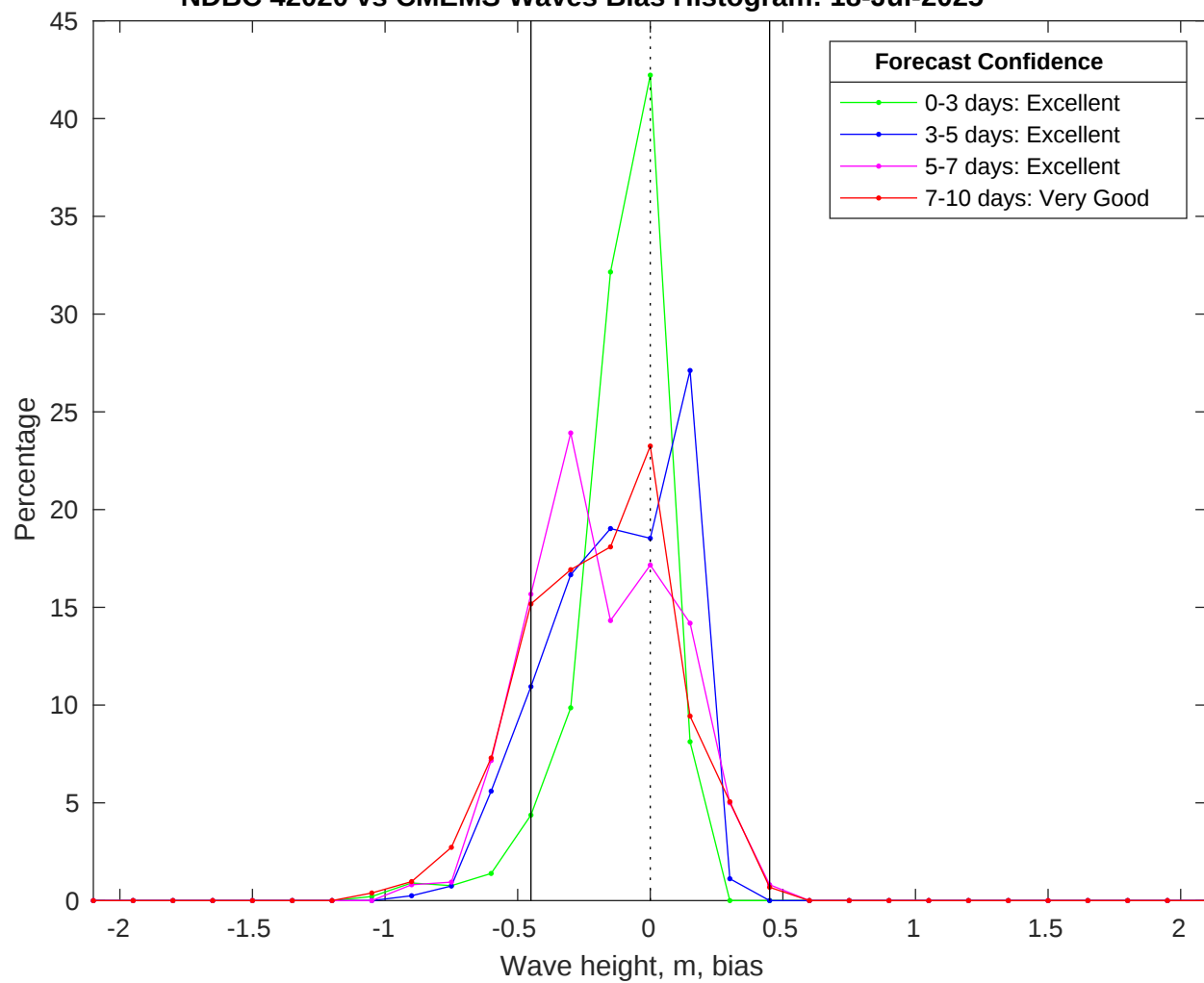
NDBC 42020 vs CMEMS Waves Bias Histogram: 18-Jul-2025
