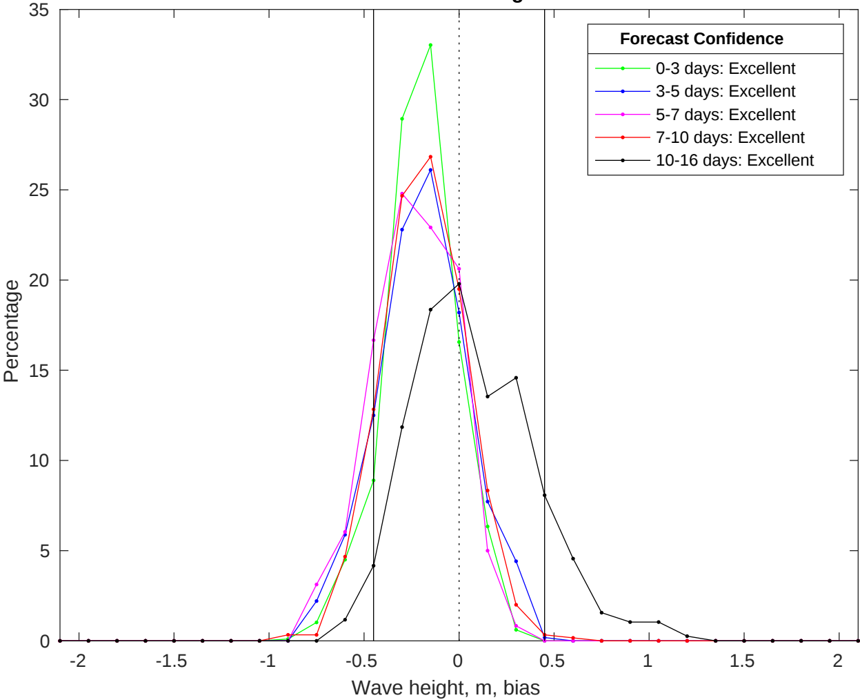
NDBC 42020 vs GFS Waves Bias Histogram: 18-Jul-2025
