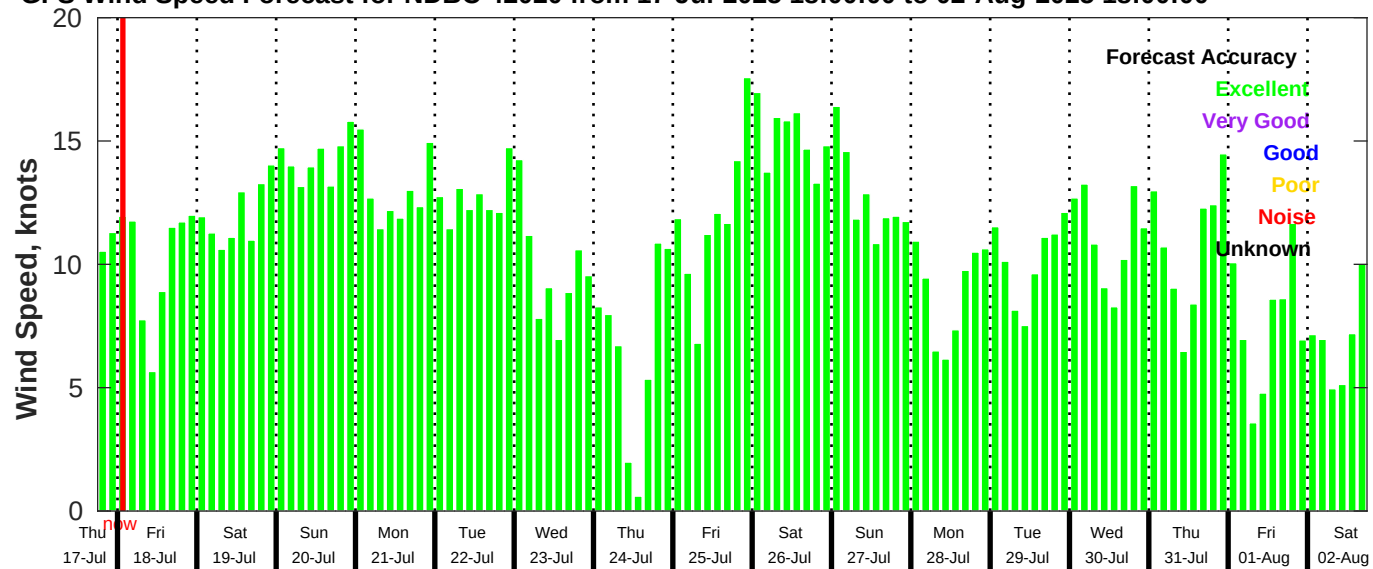
GFS Wind Speed Forecast for NDBC 42020 from 17-Jul-2025 18:00:00 to 02-Aug-2025 18:00:00
