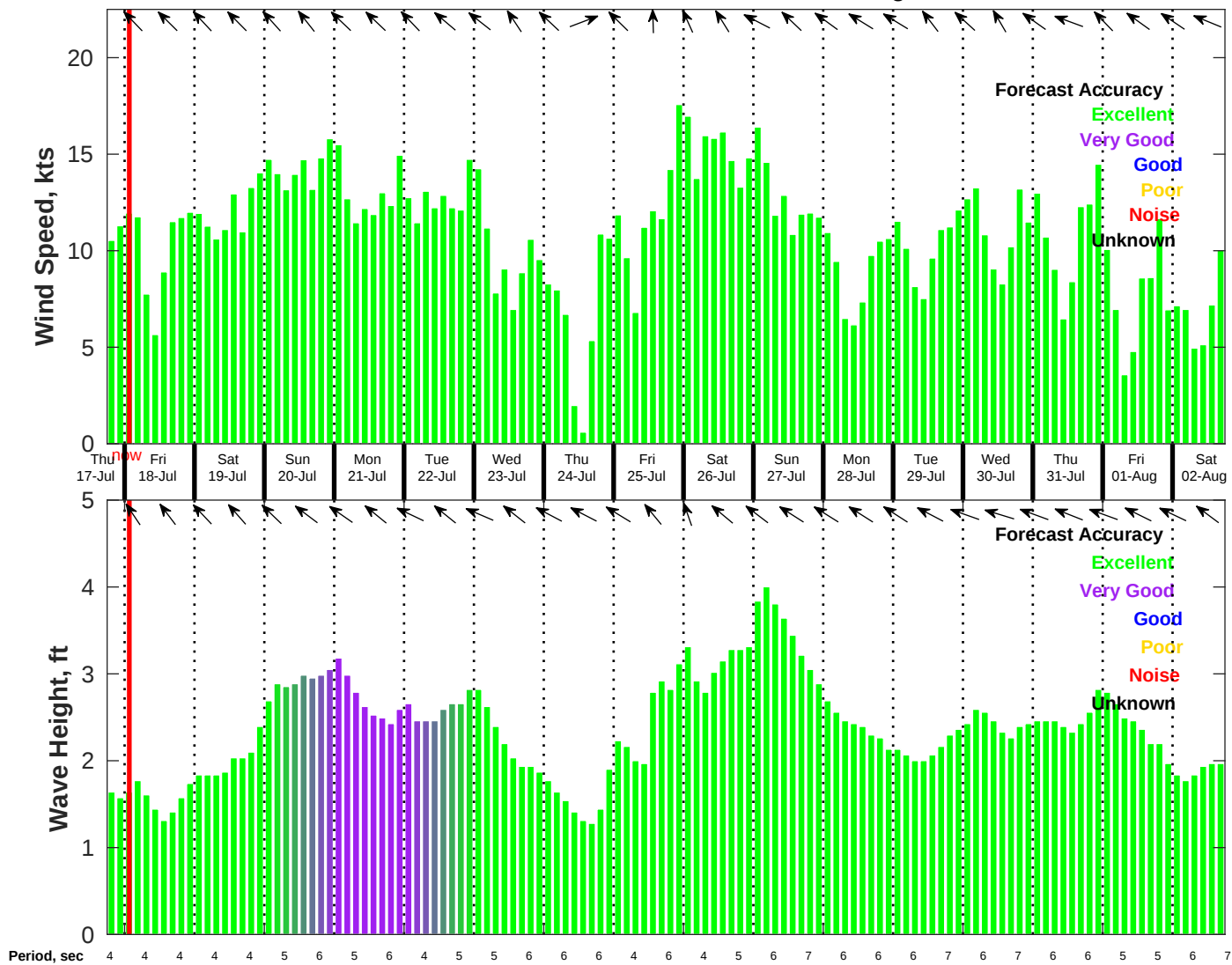
Wind & Wave Forecast for NDBC 42020 from 17-Jul-2025 18:00:00 to 02-Aug-2025 18:00:00
