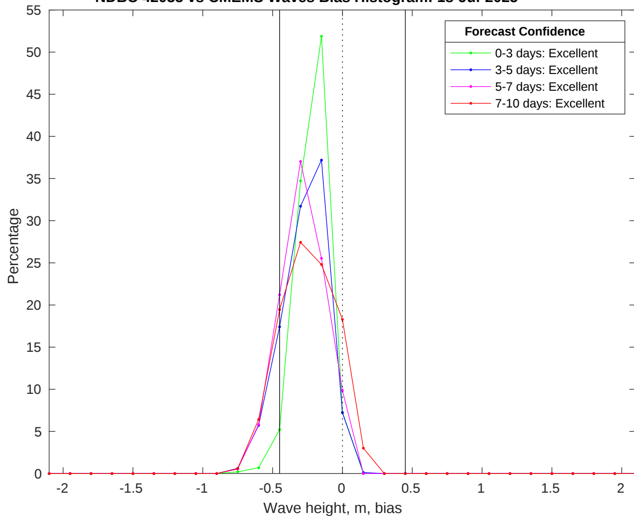
NDBC 42035 vs CMEMS Waves Bias Histogram: 18-Jul-2025
