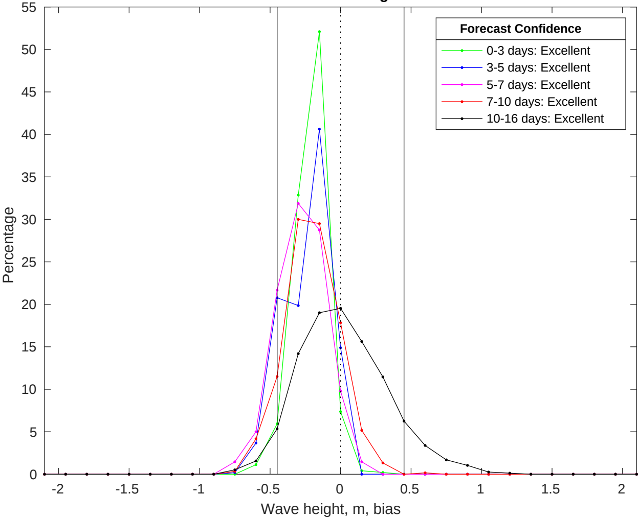
NDBC 42035 vs GFS Waves Bias Histogram: 18-Jul-2025
