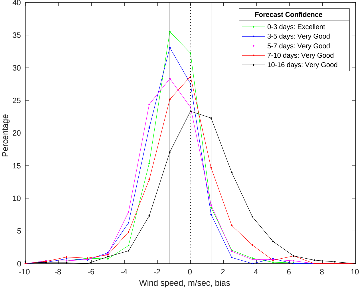
NDBC 42035 vs GFS Winds Bias Histogram: 18-Jul-2025
