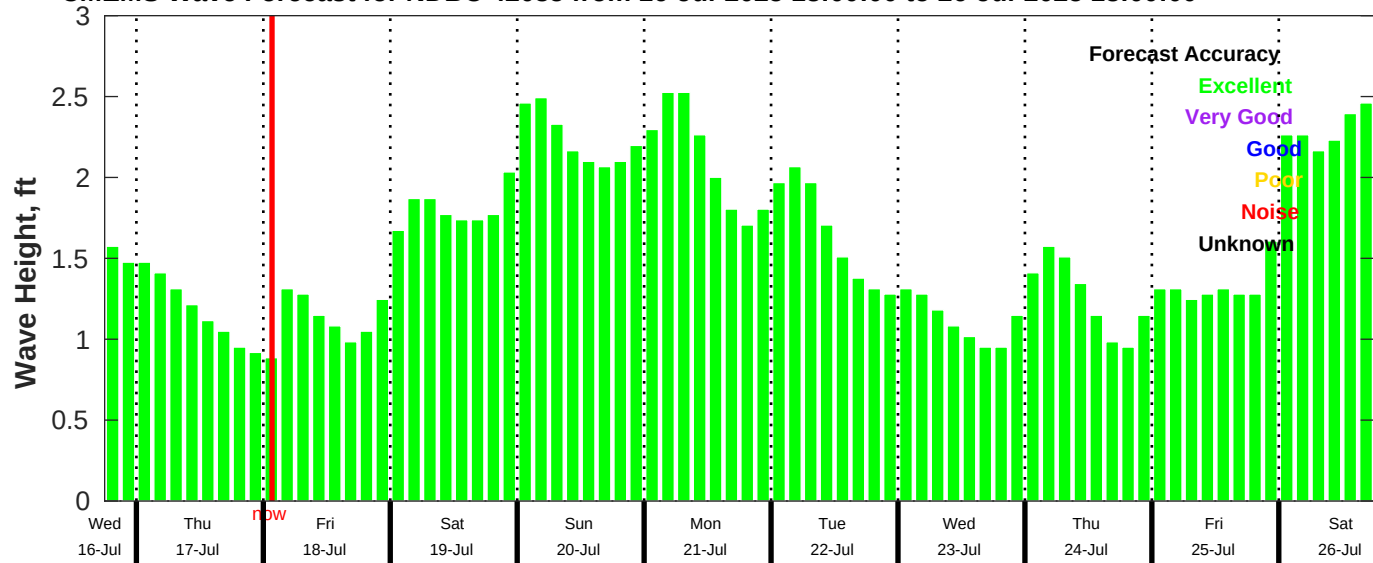
CMEMS Wave Forecast for NDBC 42035 from 16-Jul-2025 18:00:00 to 26-Jul-2025 18:00:00
