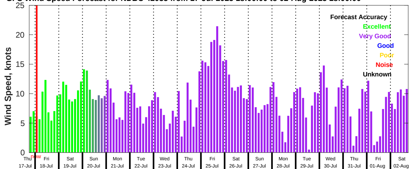
GFS Wind Speed Forecast for NDBC 42035 from 17-Jul-2025 18:00:00 to 02-Aug-2025 18:00:00
