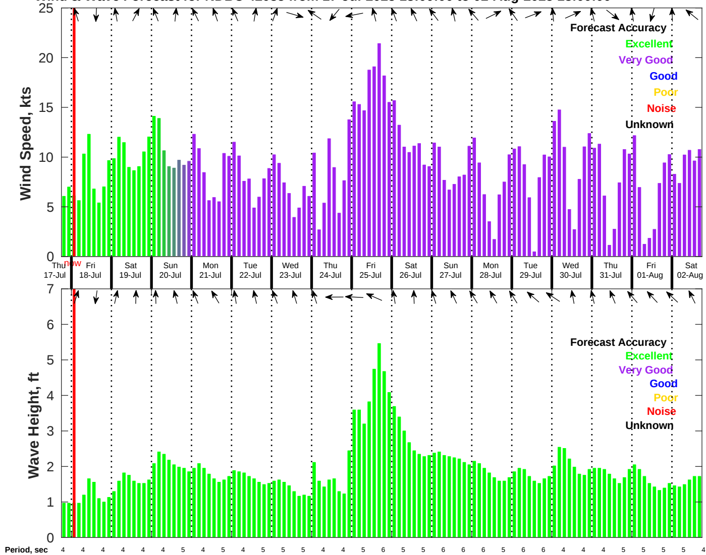
Wind & Wave Forecast for NDBC 42035 from 17-Jul-2025 18:00:00 to 02-Aug-2025 18:00:00
