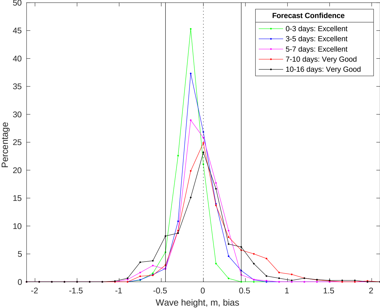
NDBC 42036 vs GFS Waves Bias Histogram: 18-Jul-2025
