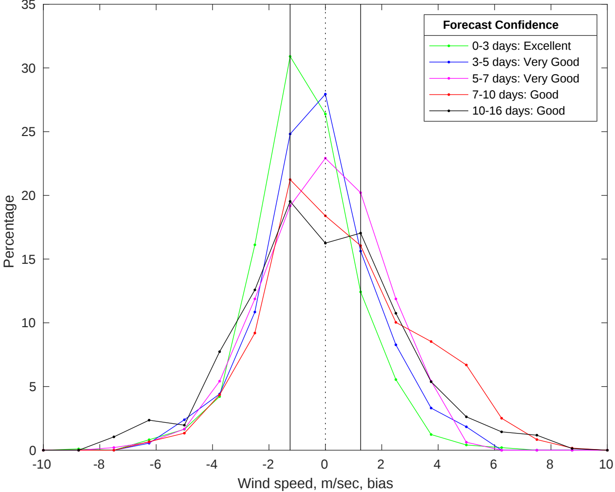
NDBC 42036 vs GFS Winds Bias Histogram: 18-Jul-2025
