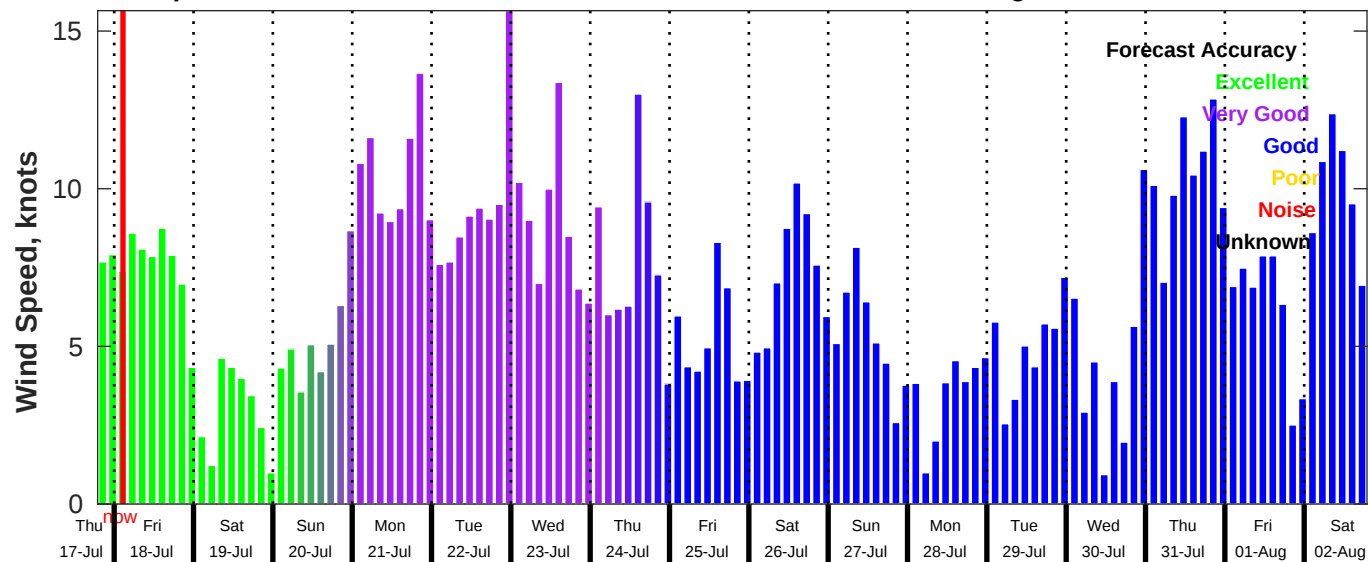
GFS Wind Speed Forecast for NDBC 42036 from 17-Jul-2025 19:00:00 to 02-Aug-2025 19:00:00
