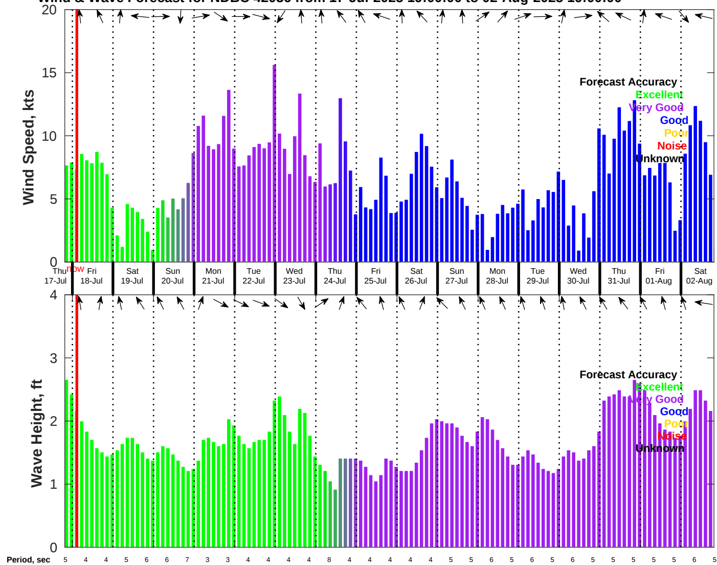
Wind & Wave Forecast for NDBC 42036 from 17-Jul-2025 19:00:00 to 02-Aug-2025 19:00:00
