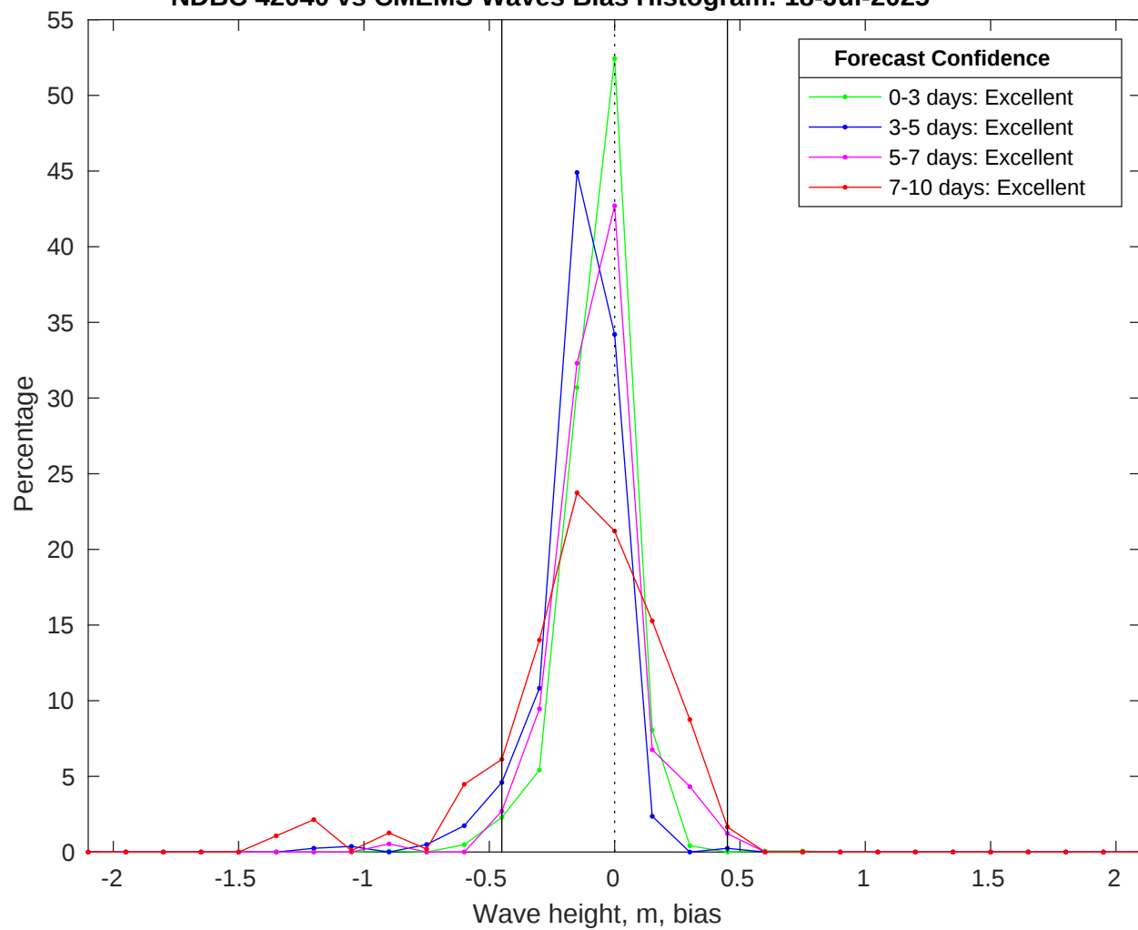
NDBC 42040 vs CMEMS Waves Bias Histogram: 18-Jul-2025
