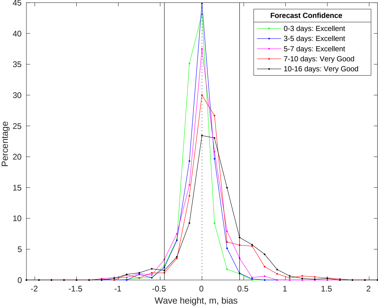
NDBC 42040 vs GFS Waves Bias Histogram: 18-Jul-2025
