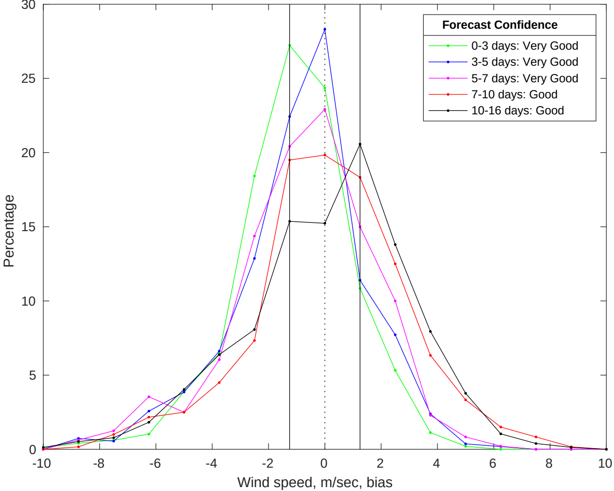
NDBC 42040 vs GFS Winds Bias Histogram: 18-Jul-2025
