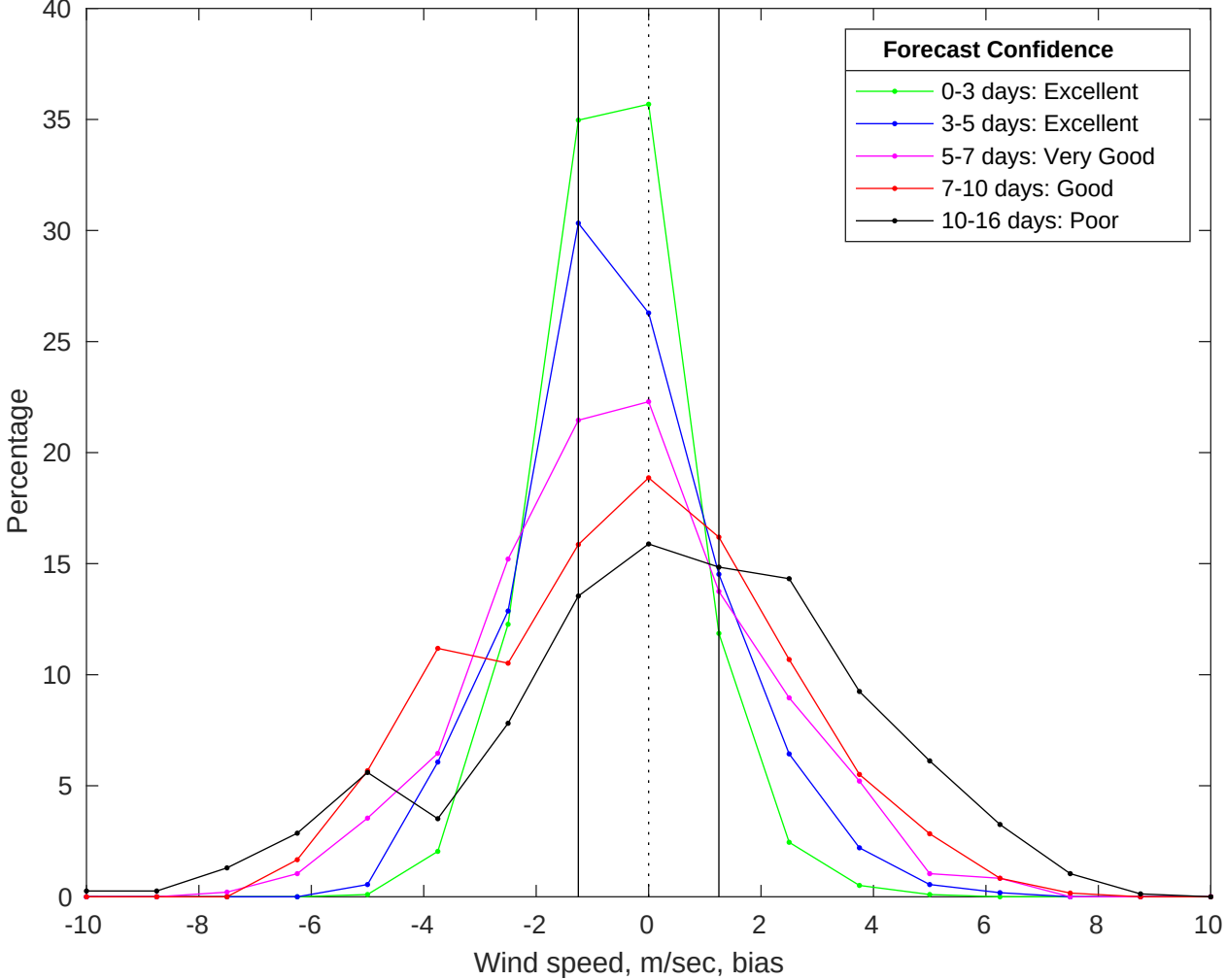
NDBC 46011 vs GFS Winds Bias Histogram: 18-Jul-2025
