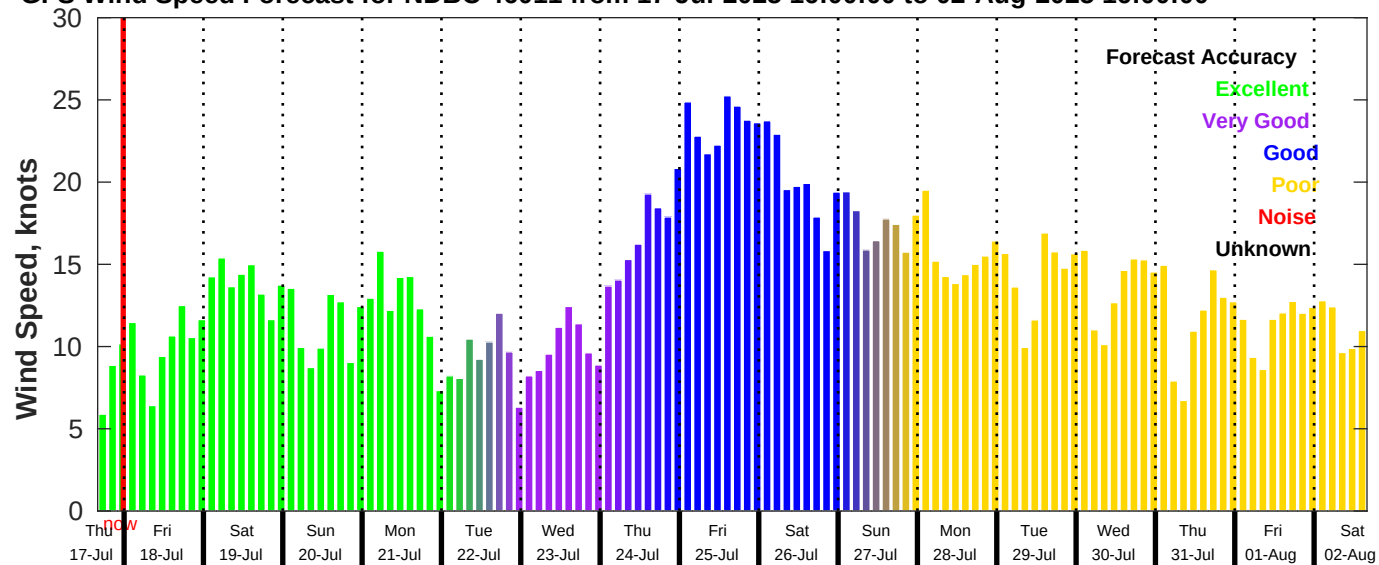
GFS Wind Speed Forecast for NDBC 46011 from 17-Jul-2025 16:00:00 to 02-Aug-2025 16:00:00
