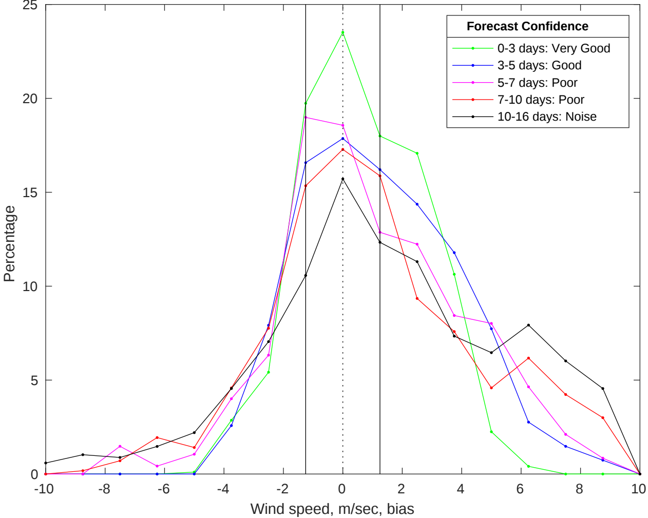
NDBC 46028 vs GFS Winds Bias Histogram: 18-Jul-2025
