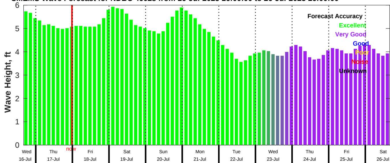
CMEMS Wave Forecast for NDBC 46028 from 16-Jul-2025 16:00:00 to 26-Jul-2025 16:00:00
