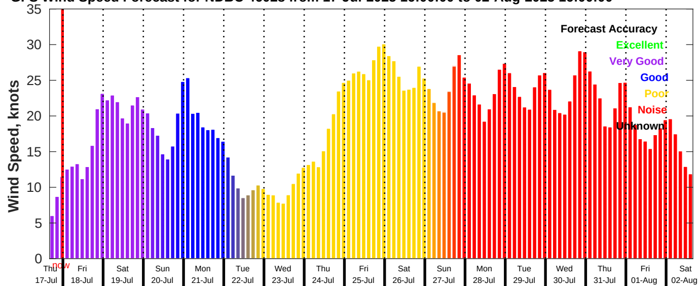
GFS Wind Speed Forecast for NDBC 46028 from 17-Jul-2025 16:00:00 to 02-Aug-2025 16:00:00
