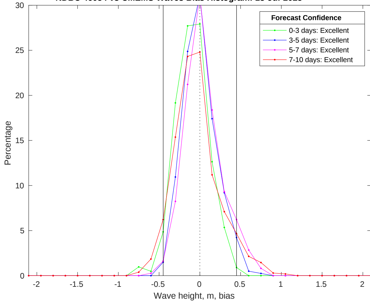
NDBC 46054 vs CMEMS Waves Bias Histogram: 18-Jul-2025
