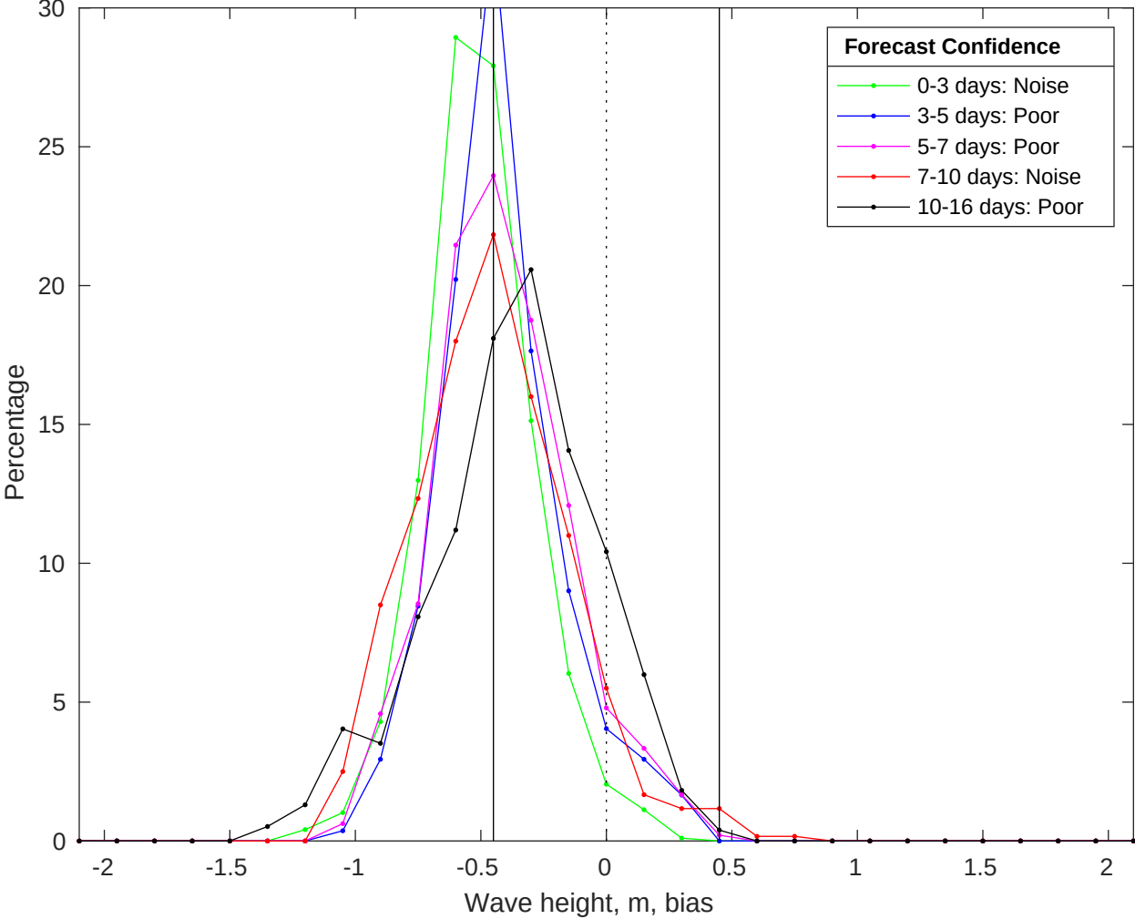
NDBC 46054 vs GFS Waves Bias Histogram: 18-Jul-2025
