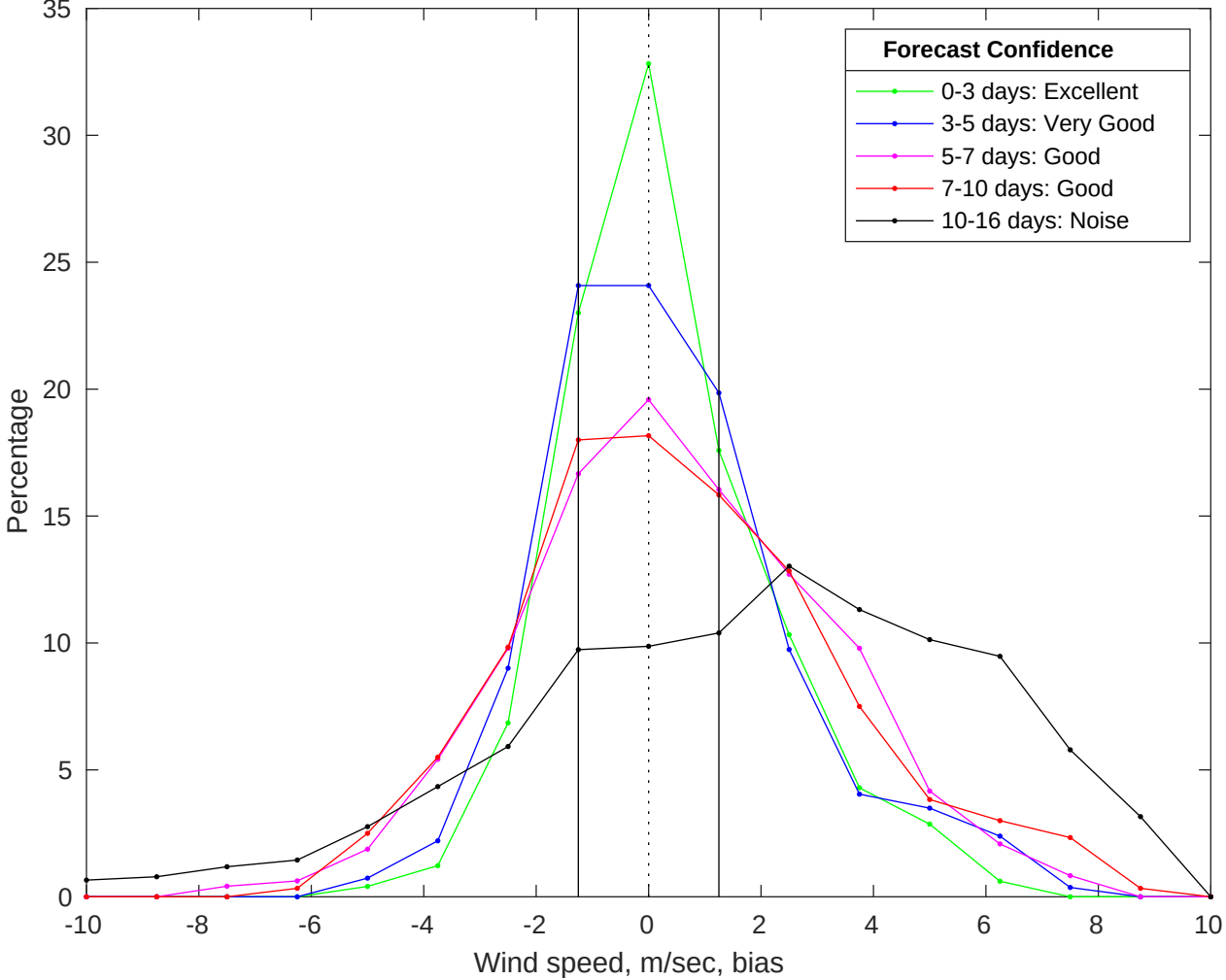
NDBC 46054 vs GFS Winds Bias Histogram: 18-Jul-2025
