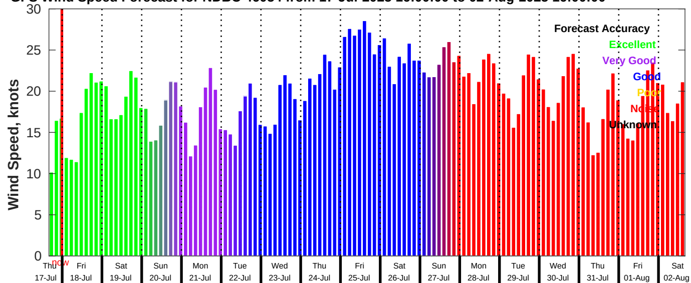
GFS Wind Speed Forecast for NDBC 46054 from 17-Jul-2025 16:00:00 to 02-Aug-2025 16:00:00
