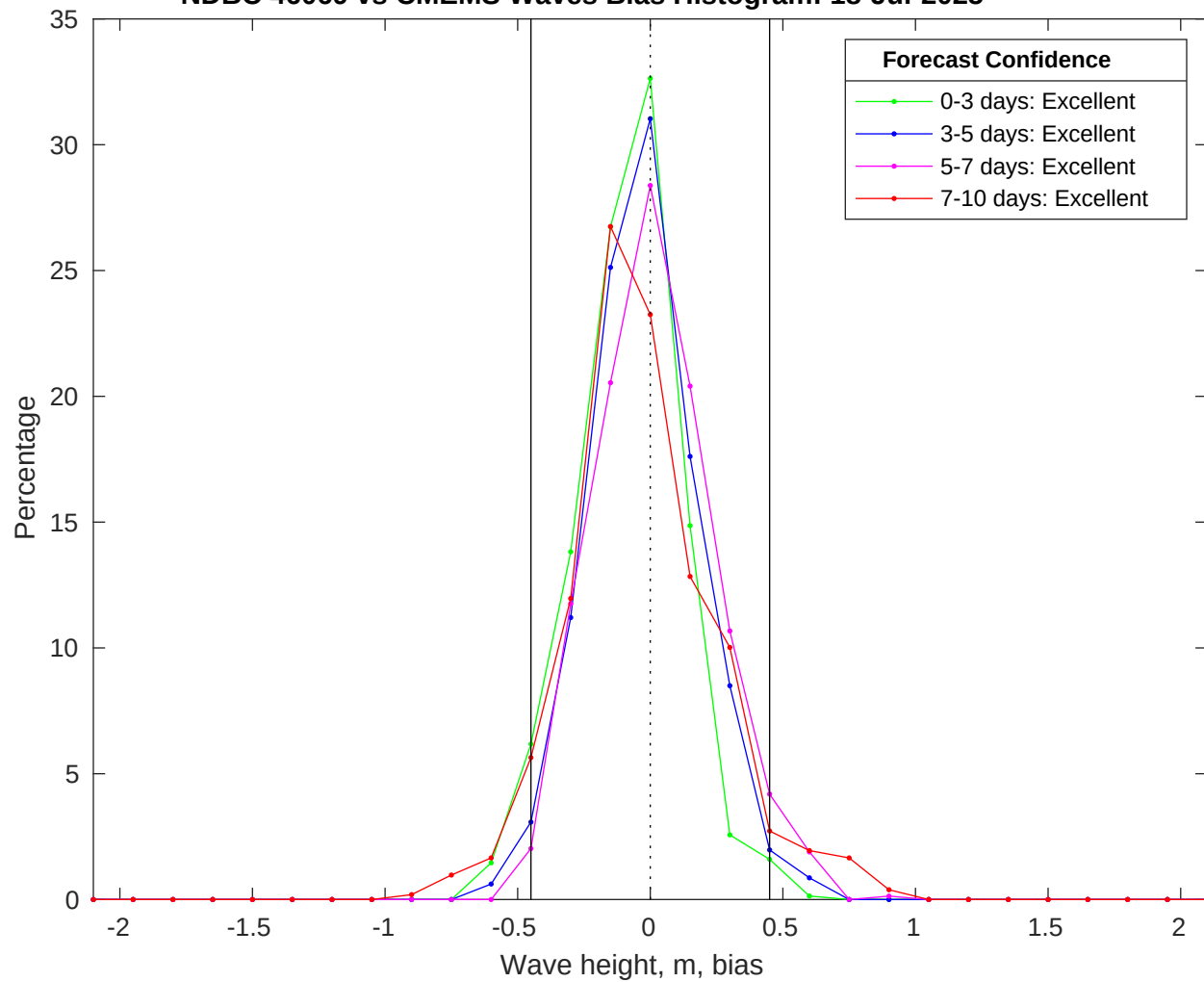
NDBC 46069 vs CMEMS Waves Bias Histogram: 18-Jul-2025
