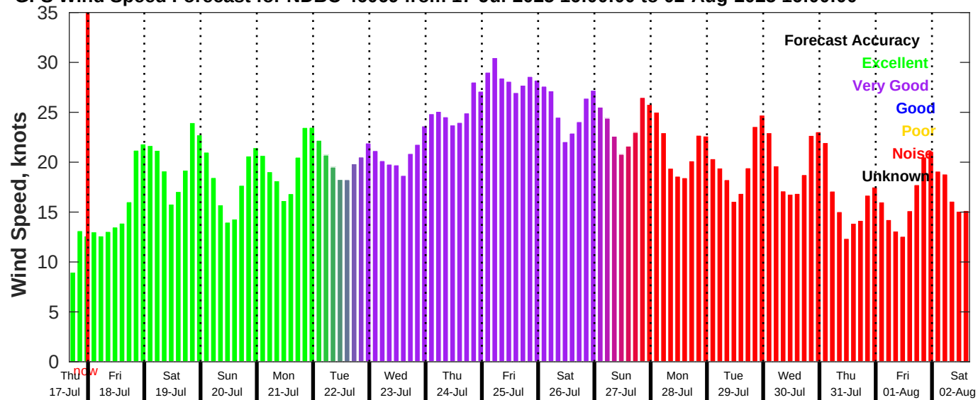
GFS Wind Speed Forecast for NDBC 46069 from 17-Jul-2025 16:00:00 to 02-Aug-2025 16:00:00
