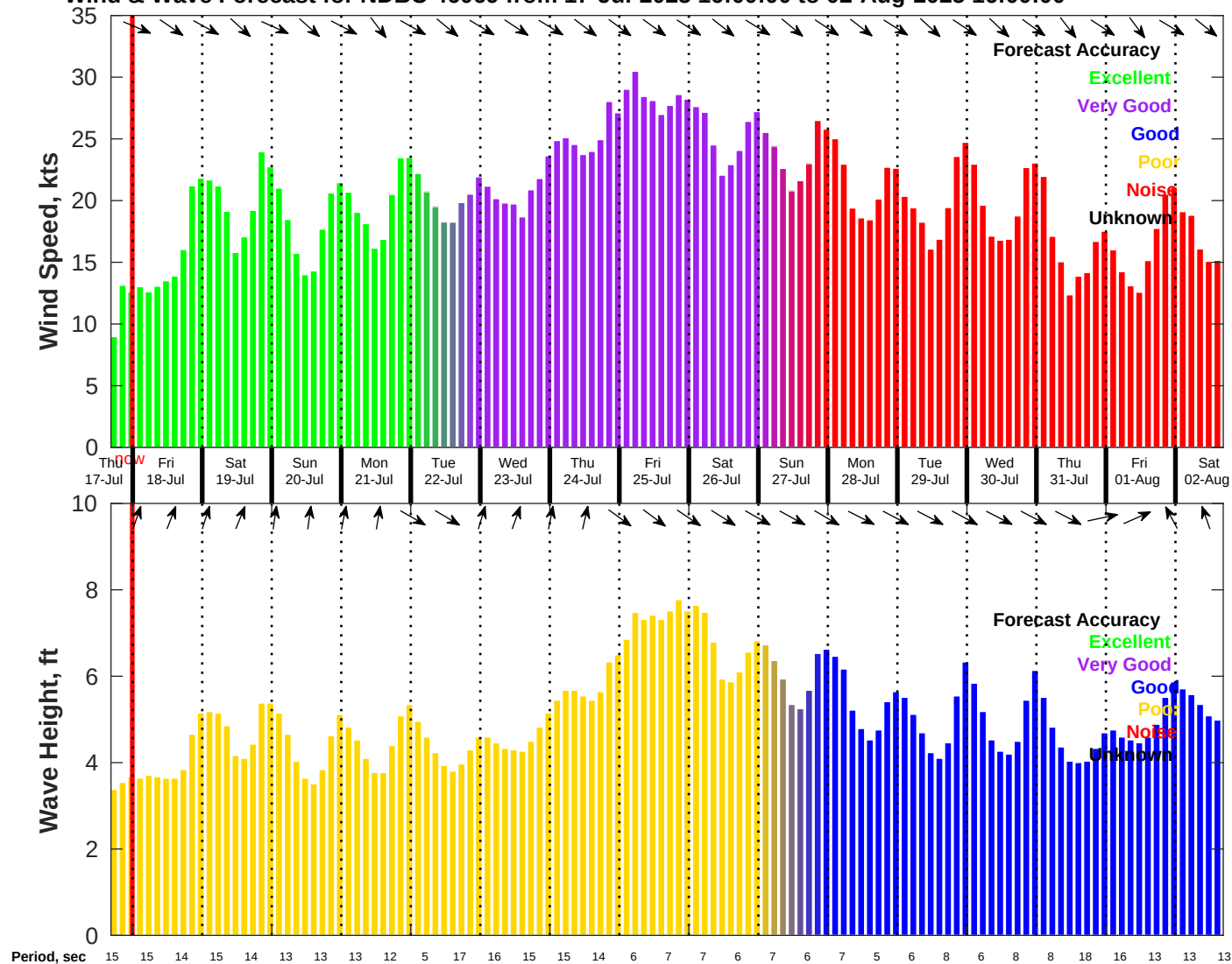
Wind & Wave Forecast for NDBC 46069 from 17-Jul-2025 16:00:00 to 02-Aug-2025 16:00:00
