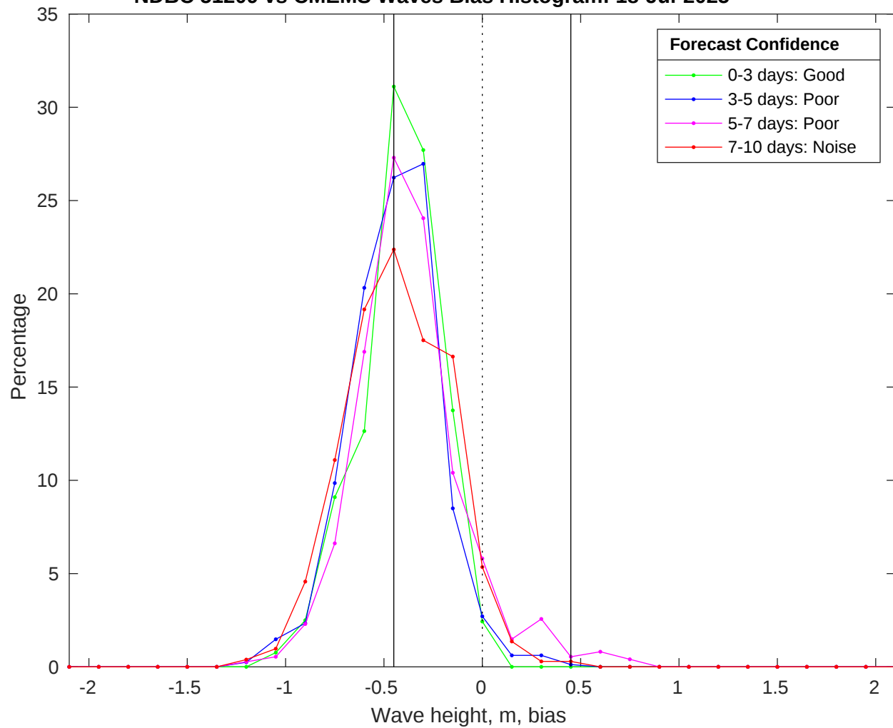
NDBC 51209 vs CMEMS Waves Bias Histogram: 18-Jul-2025
