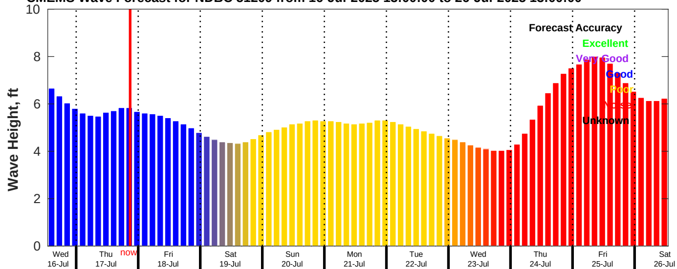
CMEMS Wave Forecast for NDBC 51209 from 16-Jul-2025 13:00:00 to 26-Jul-2025 13:00:00
