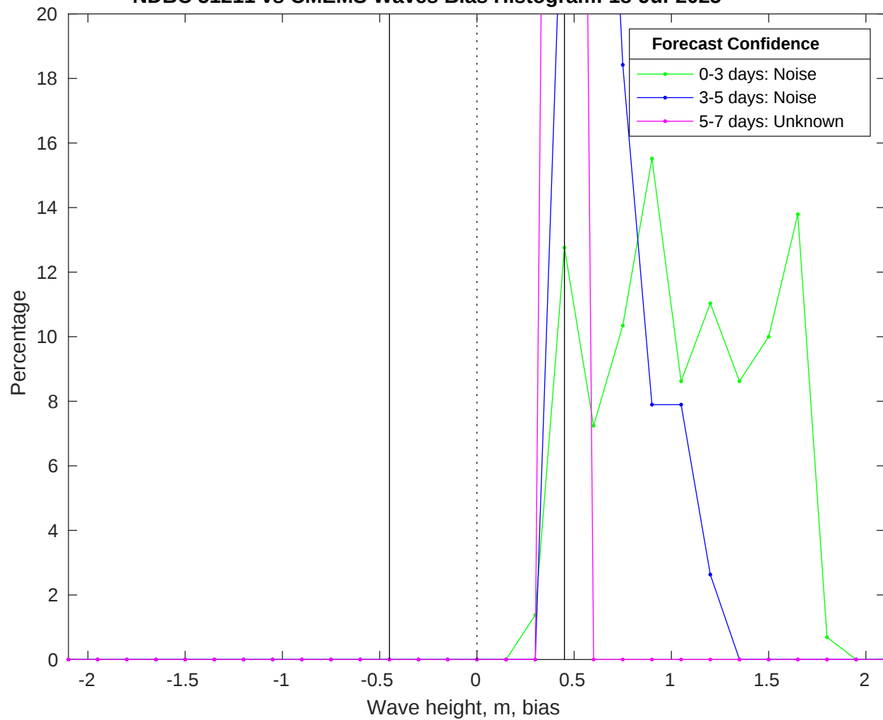
NDBC 51211 vs CMEMS Waves Bias Histogram: 18-Jul-2025
