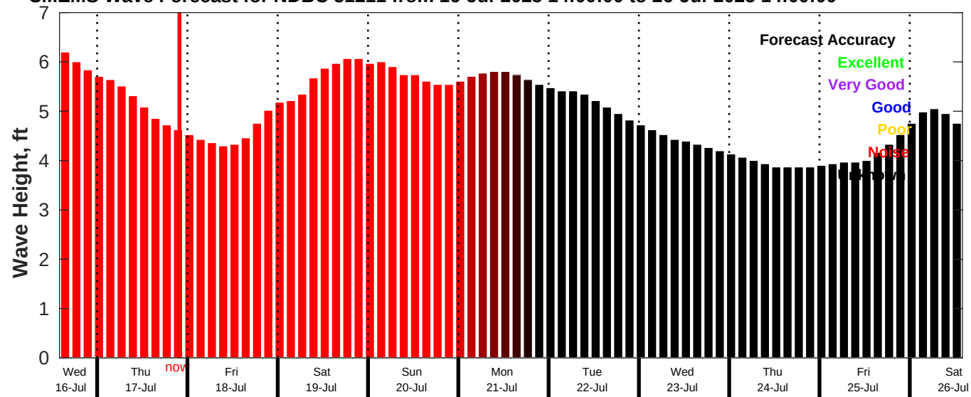
CMEMS Wave Forecast for NDBC 51211 from 16-Jul-2025 14:00:00 to 26-Jul-2025 14:00:00
