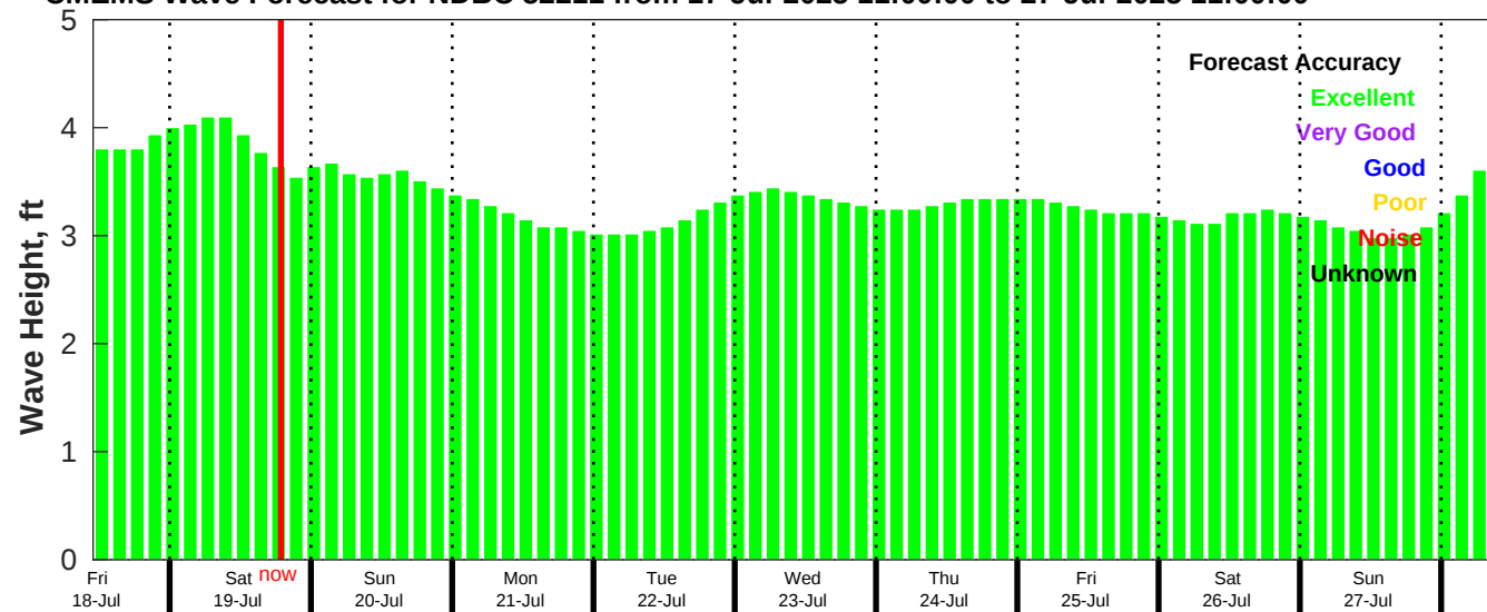
CMEMS Wave Forecast for NDBC 52211 from 17-Jul-2025 11:00:00 to 27-Jul-2025 11:00:00
