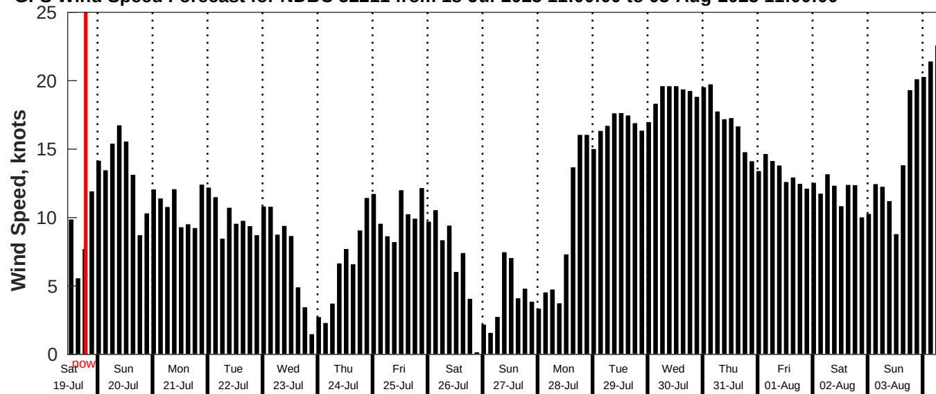
GFS Wind Speed Forecast for NDBC 52211 from 18-Jul-2025 11:00:00 to 03-Aug-2025 11:00:00
