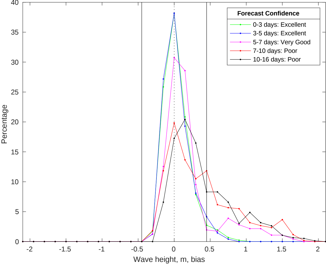
NDBC 52212 vs GFS Waves Bias Histogram: 18-Jul-2025
