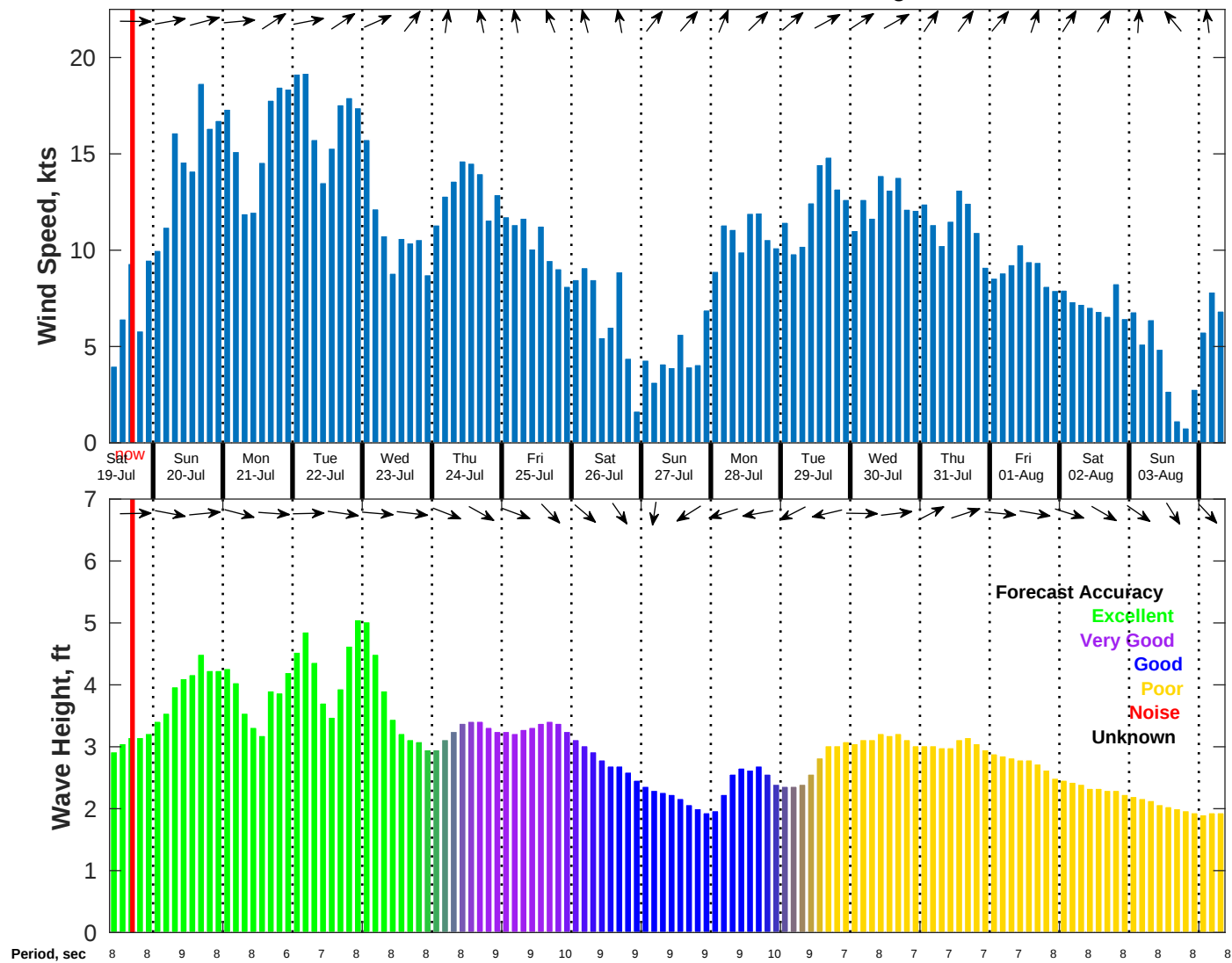
Wind & Wave Forecast for NDBC 52212 from 18-Jul-2025 09:00:00 to 03-Aug-2025 09:00:00
