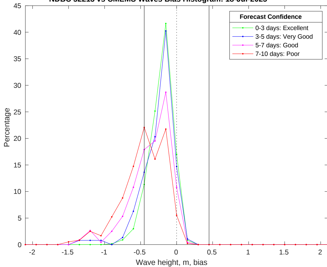
NDBC 52213 vs CMEMS Waves Bias Histogram: 18-Jul-2025
