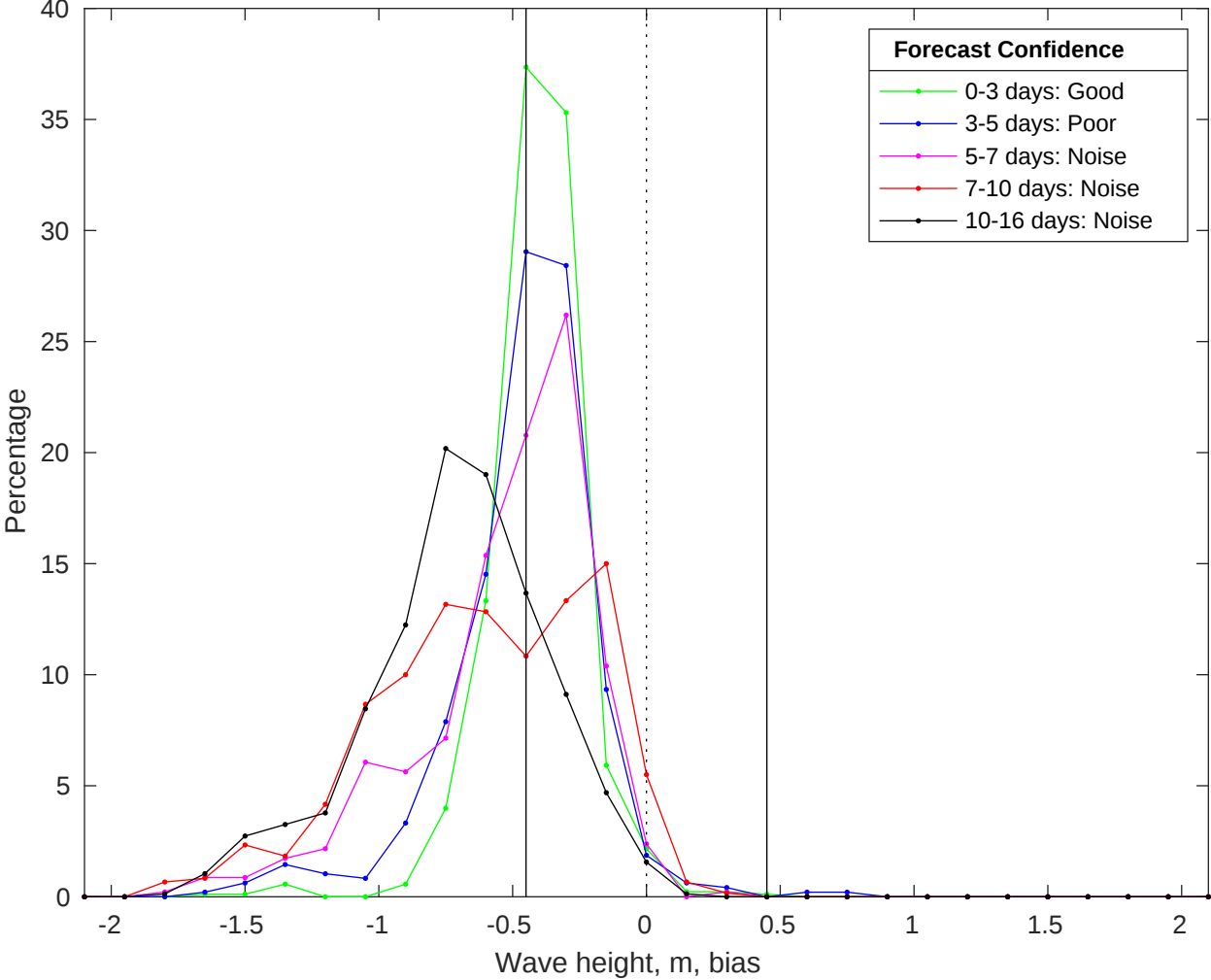
NDBC 52213 vs GFS Waves Bias Histogram: 18-Jul-2025
