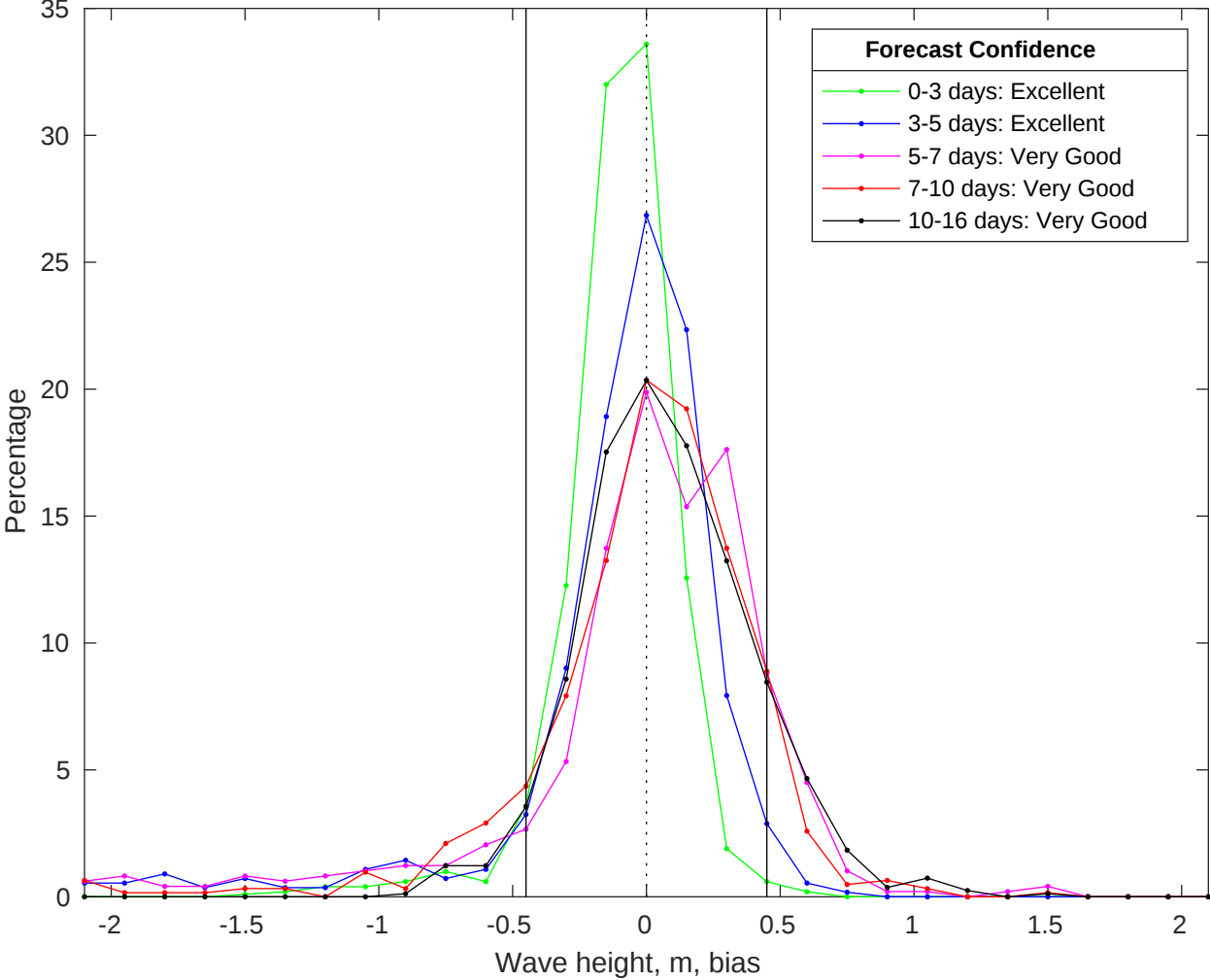
NDBC 41004 vs GFS Waves Bias Histogram: 19-Jul-2025
