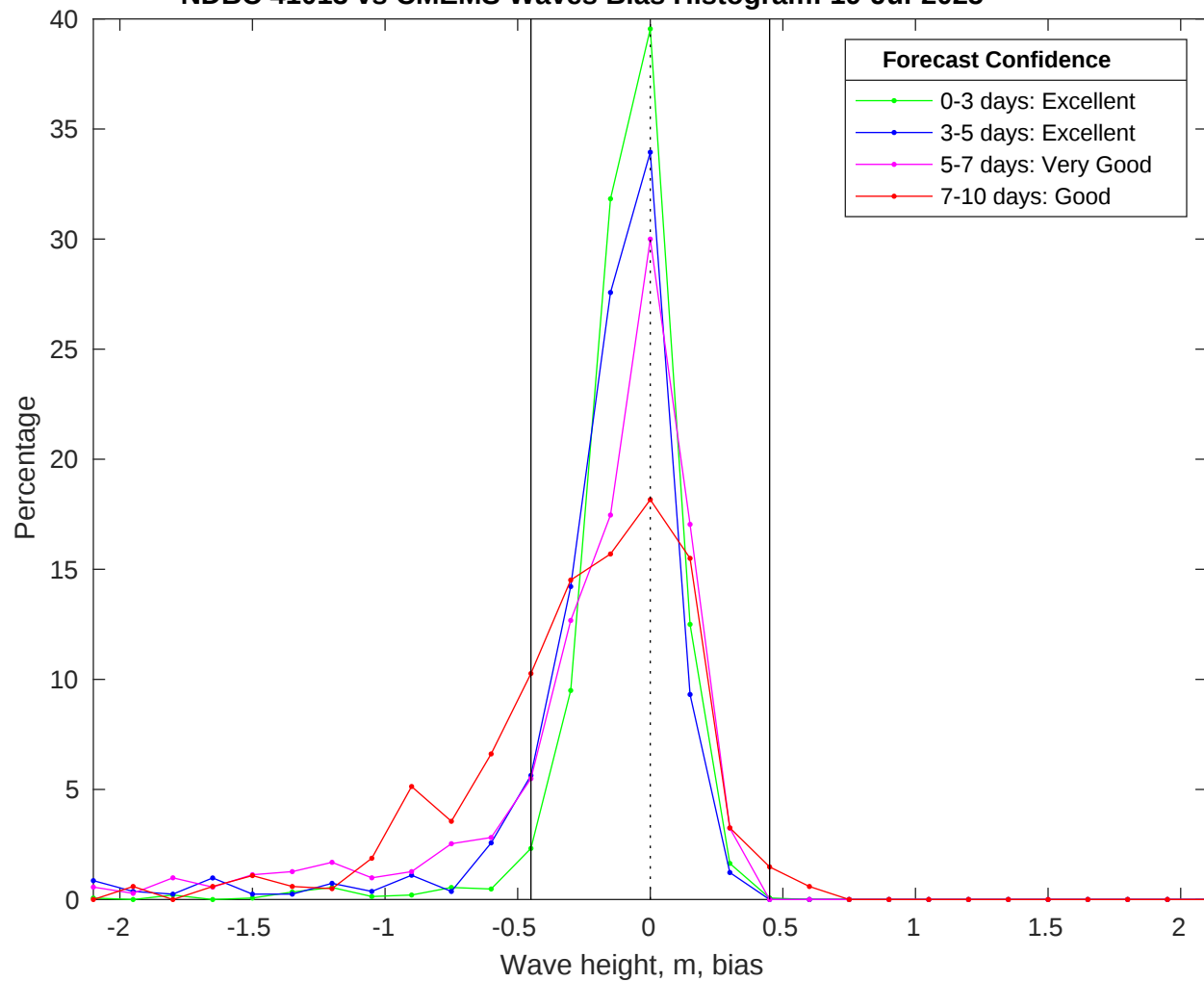
NDBC 41013 vs CMEMS Waves Bias Histogram: 19-Jul-2025
