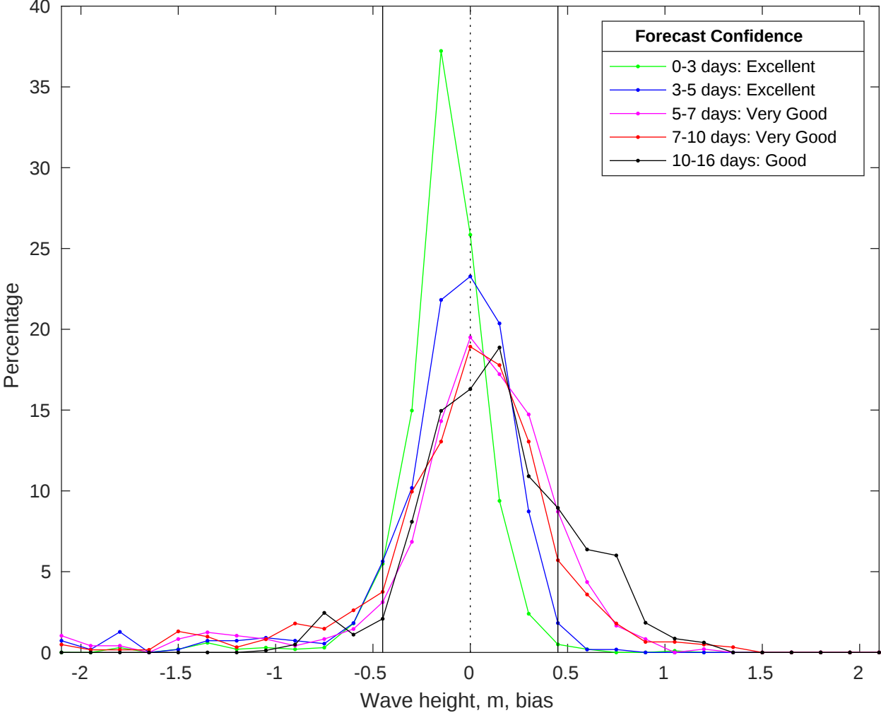
NDBC 41013 vs GFS Waves Bias Histogram: 19-Jul-2025
