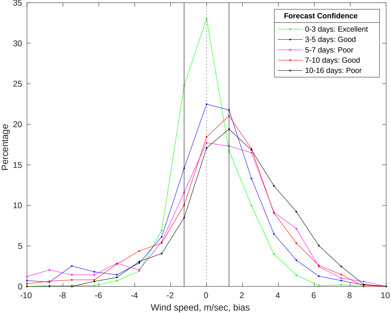
NDBC 41013 vs GFS Winds Bias Histogram: 19-Jul-2025
