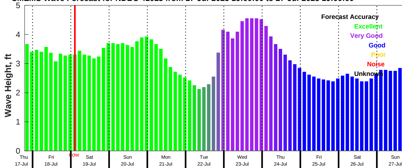
CMEMS Wave Forecast for NDBC 41013 from 17-Jul-2025 19:00:00 to 27-Jul-2025 19:00:00
