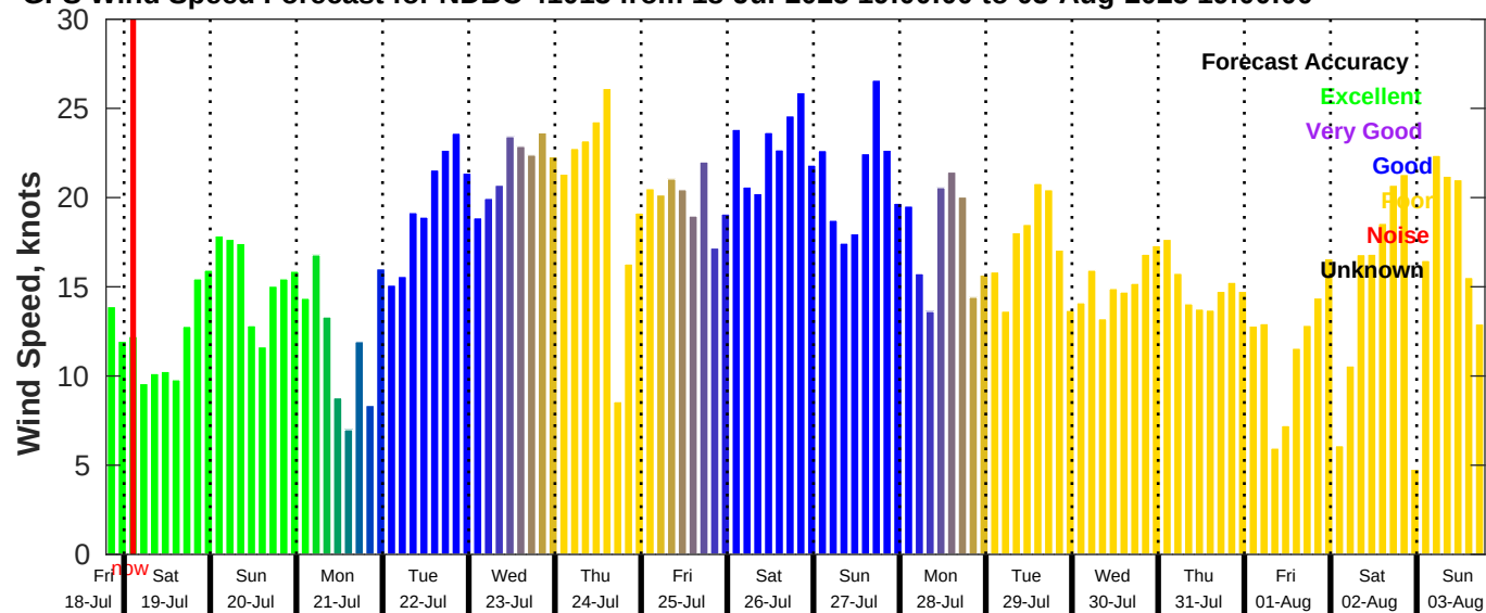
GFS Wind Speed Forecast for NDBC 41013 from 18-Jul-2025 19:00:00 to 03-Aug-2025 19:00:00
