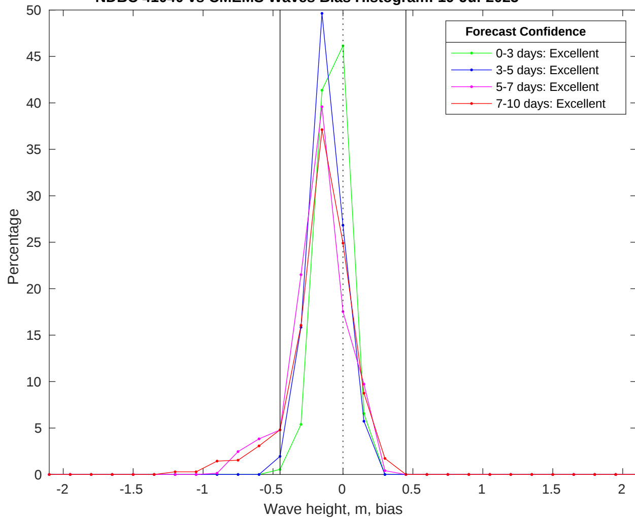
NDBC 41040 vs CMEMS Waves Bias Histogram: 19-Jul-2025
