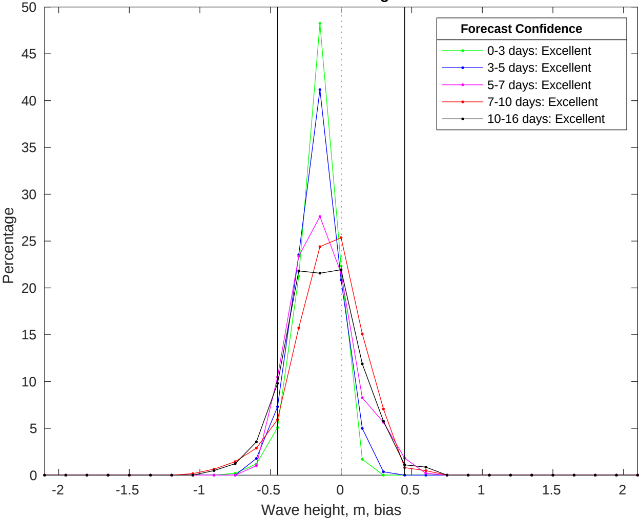
NDBC 41040 vs GFS Waves Bias Histogram: 19-Jul-2025
