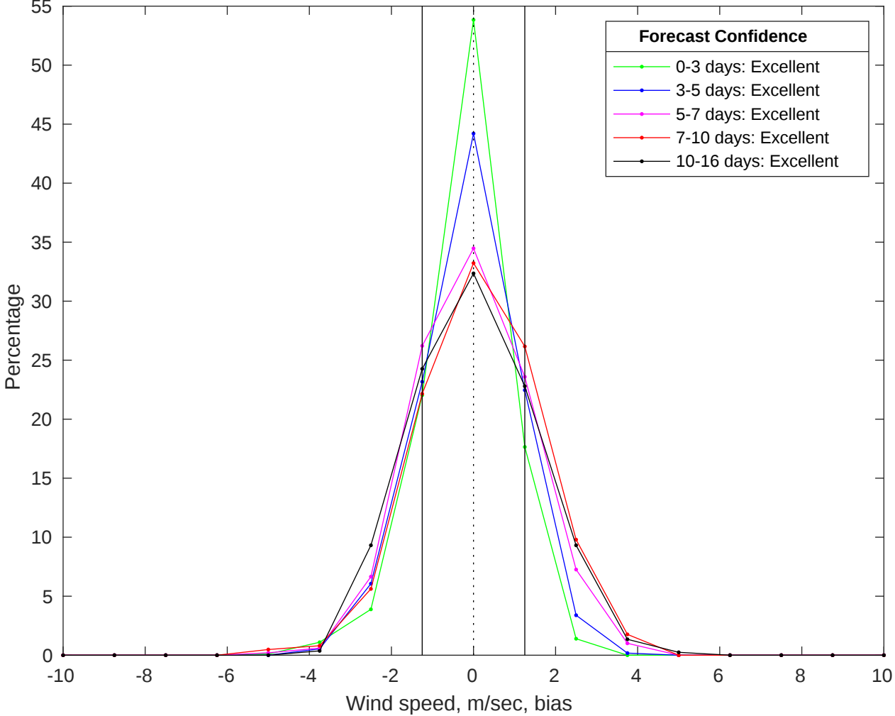
NDBC 41040 vs GFS Winds Bias Histogram: 19-Jul-2025
